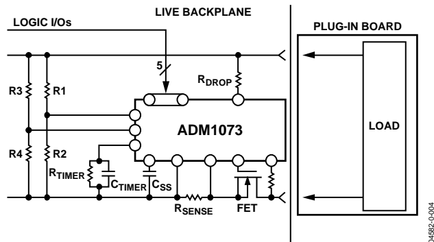
Figure 4. ADM1073 Residing on a Backplane
